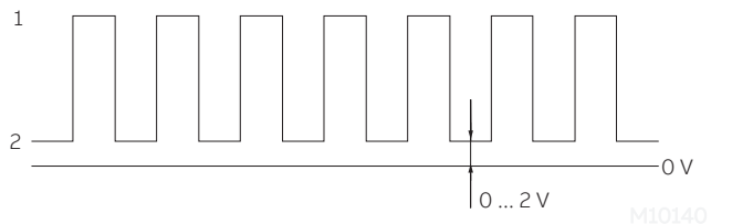
Figure 2: High and low level (pulse output)
