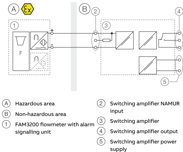
Figure 13: Electrical connection of an alarm signalling unit to a switching amplifier (example)
